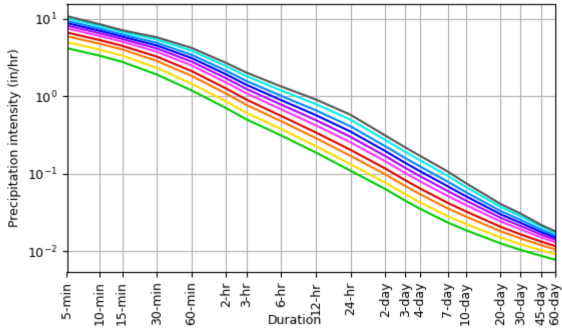
PDS-based intensity-duration-frequency (IDF) curves Latitude: 38.9428°, Longitude: -76.9329°
